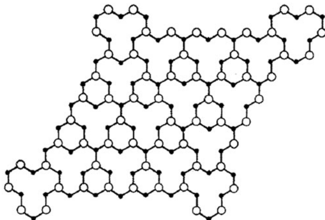
Figure 4. The topmost atoms of the Lander vacancy model of the 7\times 7 , based on an interpretation of LEED images like the one in Figure 3. Reprinted with permission from J.J. Lander and J. Morrison, 'Structures of clean surfaces of silicon and germanium', Journal of Applied Physics (1963) 34, pp. 1403–1410, p. 1410, copyright (1963), American Institute of Physics.
