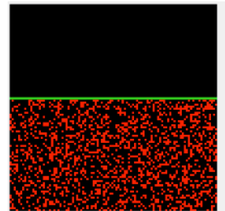
2000 “gas particles” supporting a moveable piston
