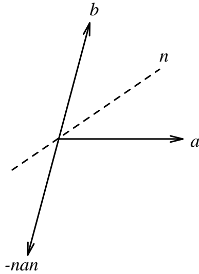
Figure 1: A rotation composed of two reflections
